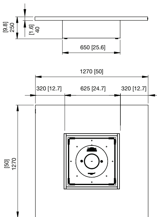
Line drawings show concrete models without a Fire Screen. Refer to the Fire Screen model specifications for dimensions.
